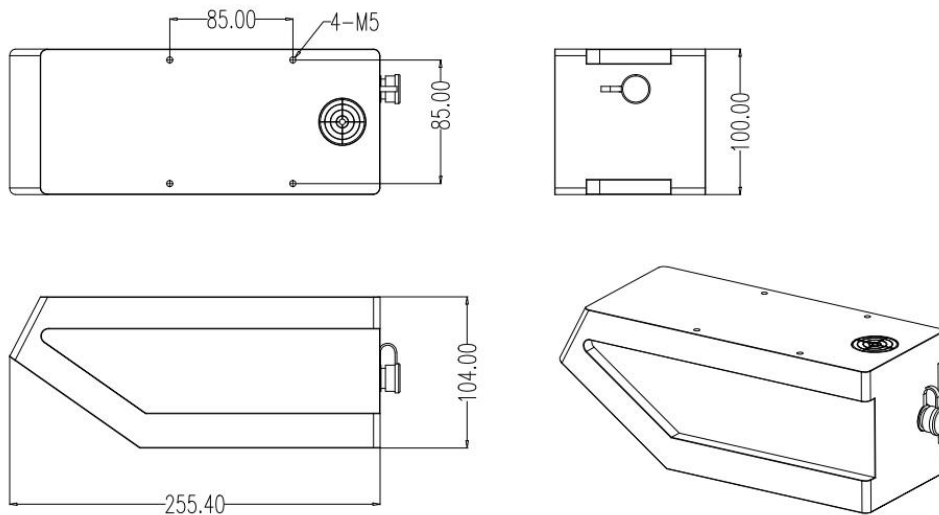
MRCM600 Dimension
