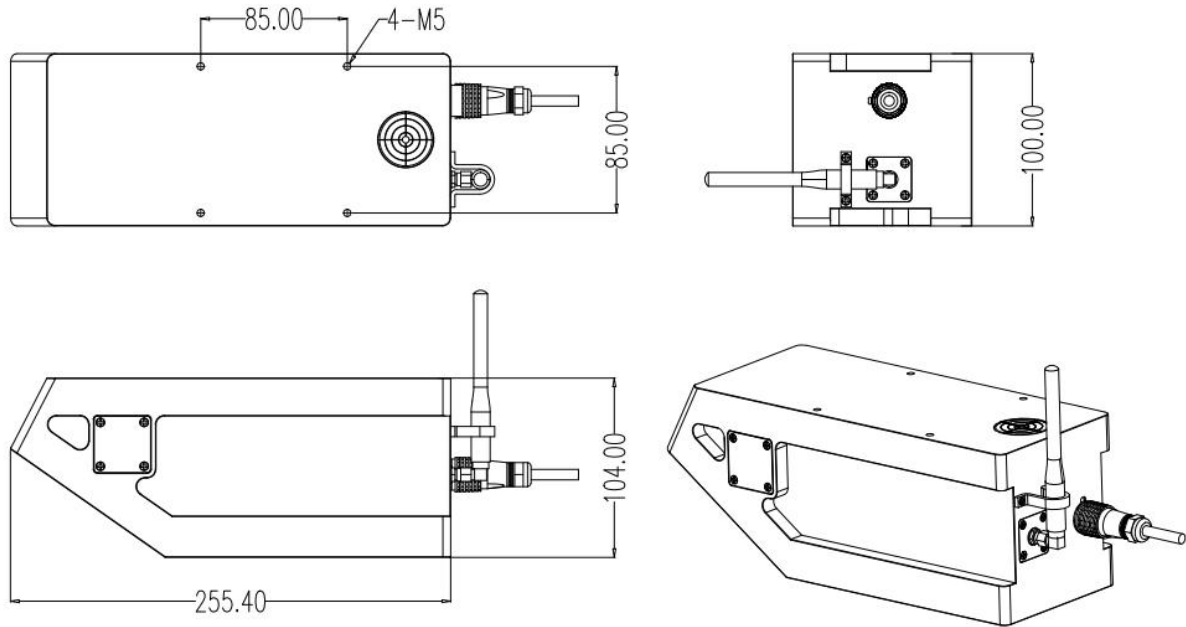
MRCM600-R dimension
